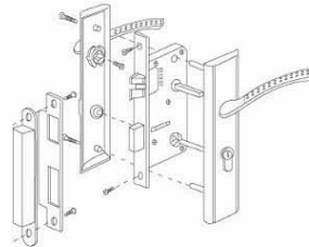
产品安装图 Installation Instruction
